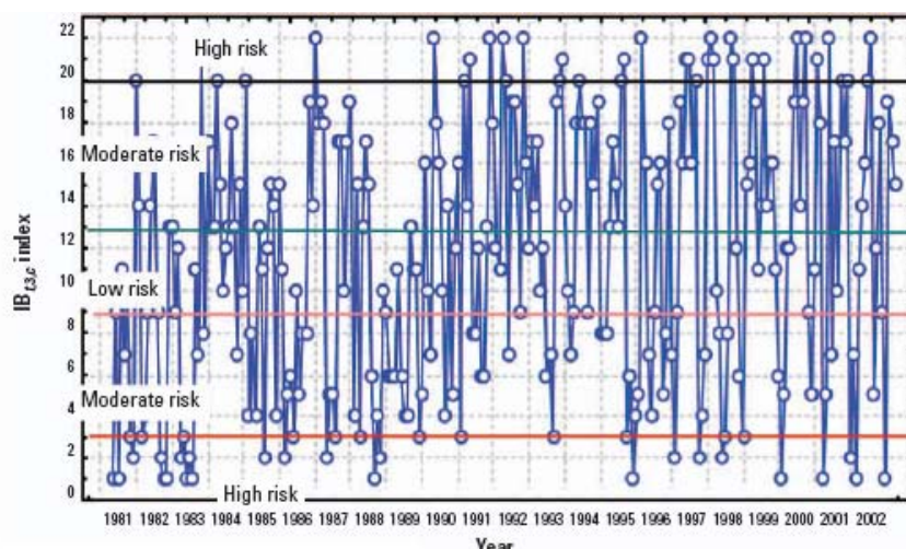
Figure 15. Risk levels using the IB_{t,3,c} index.
