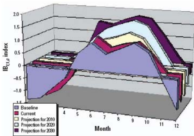
Figure 10. Climate change scenarios using the IB_{t,1,c} index.
