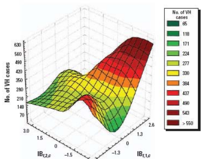
Figure 6. Association between CV and VH using the IB_{t,1,c} and IB_{t,2,c} indices.
