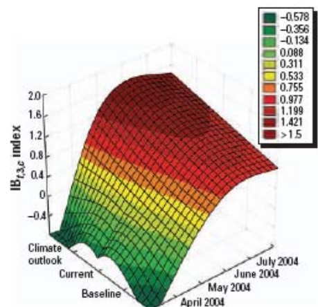
Figure 13. Baseline (1961–1990), current conditions (1991–2003), and climate outlook April–July 2004 using the IB_{t,3,c} index.
